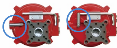
14mm Double Square Female Shaft Declutchable lever
